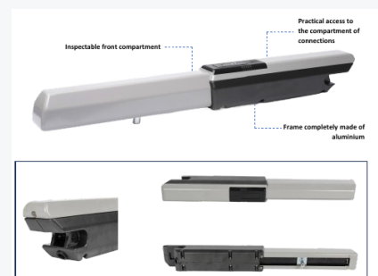
SIE 230 V arm motor — aluminium frame, inspectable compartments
